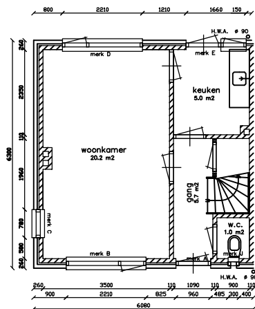
Begane-grond
