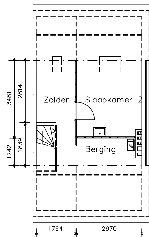
Zolder
