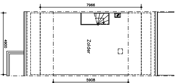
Zolder
