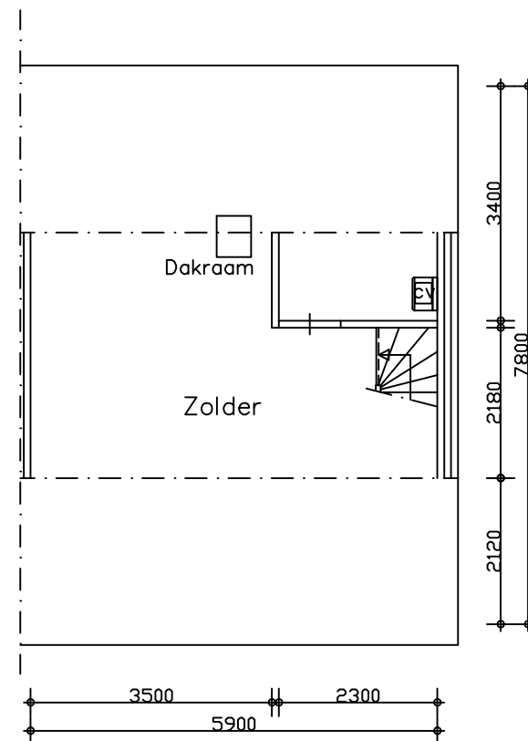
Zolder
